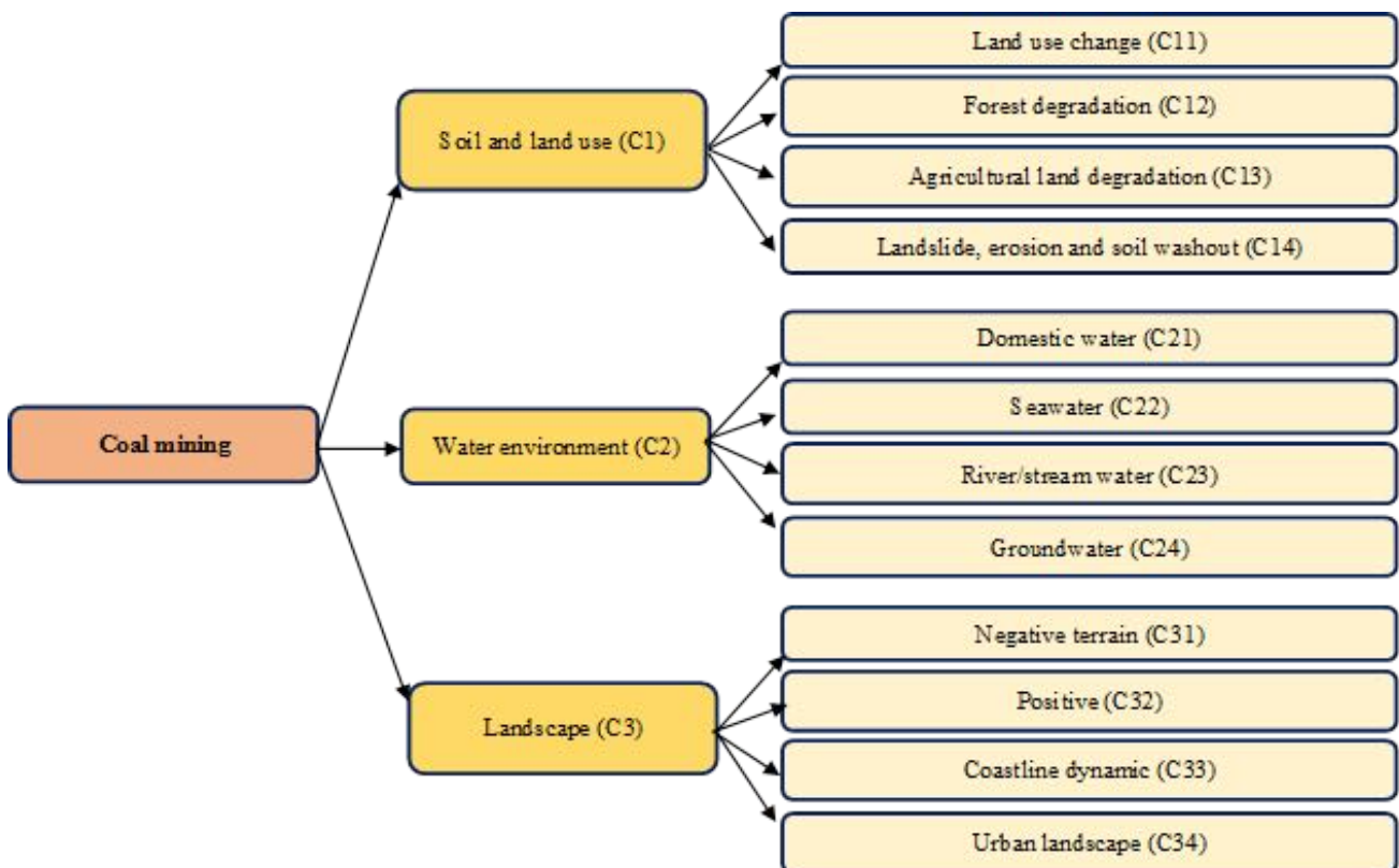
Figure 1. The variables used in AHP model
